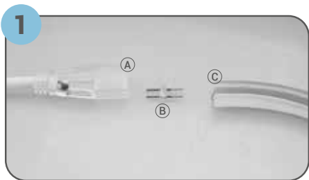
A. PLUG B. PINO C. FITA LED NEON
